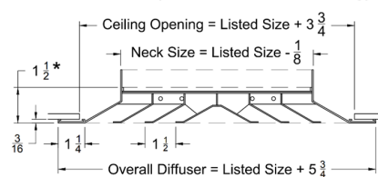
Model: 5500-1 (Flush Surface Mounting)
