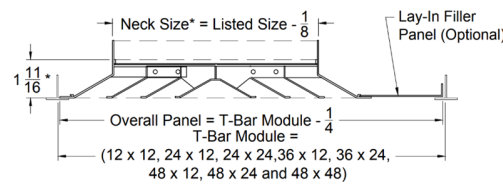
Model: 5500-6 (Lay in T-Bar)
