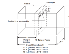
*These dimensions are furnished approximately 1/4 in. (6mm) undersize.
